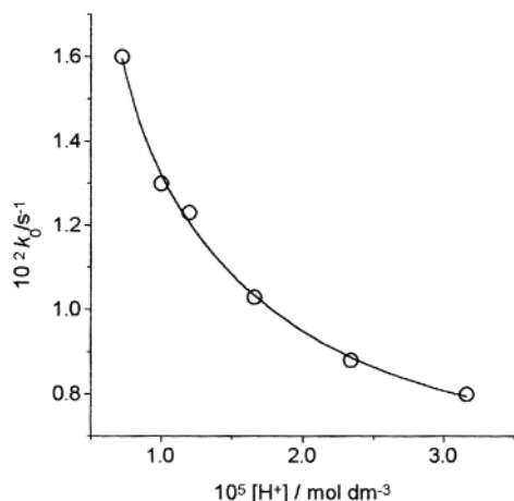
Fig. 2 Variation of k_0 with [H^+] at a fixed c_{\text{bipy}} = 5.0 \text{ mmol dm}^{-3} , [\text{complex}] = 0.1 \text{ mmol dm}^{-3} , [\text{N}_2\text{H}_5^+] = 2.0 \text{ mmol dm}^{-3} , I = 1.0 \text{ mol dm}^{-3} , T = 25.0^\circ\text{C} .
